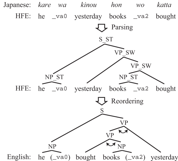
Figure 2: Example of post-ordering by parsing.
